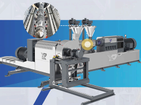
SJW 3-flight & SKW 4-flight Co-kneader
